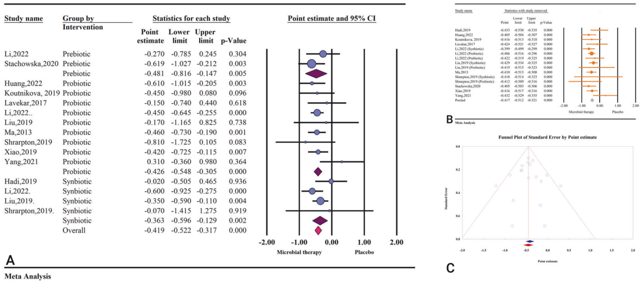
Fig. 3 The effects of microbial therapy on HOMA-IR. A Forest plot for the effect size and 95% confidential interval of gut microbial therapy on HOMA-IR in patients with NAFLD. B The results of sensitivity analysis. C The results of publication bias with three imputed studies (red dots).
