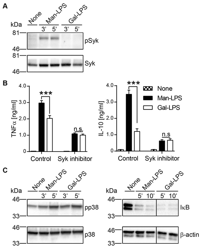
FIGURE 4. Syk-dependent BM-DC activation by Man-LPS. A, BM-DCs were stimulated with 1 \mu g/ml Man-LPS or 4 \mu g/ml Gal-LPS for the indicated time period. The stimulated cells were lysed and subjected to SDS-PAGE analysis. The proteins were transferred onto nitrocellulose membrane and analyzed for both phosphorylation and expression level of Syk. B, BM-DCs were stimulated with LPS in the presence or absence of the Syk inhibitor R406. Cytokine production was monitored by ELISA as in Fig. 1C. C, phosphorylation of p38 and degradation of I \kappa B in response to LPS were analyzed as in A. Data are representative of three independent experiments with similar results. Error bars, S.D. Statistical analyses were performed by one-way ANOVA followed by Tukey's test. ***, p < 0.001 ; n.s., not statistically significant.
