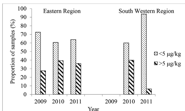
Fig. 3. Proportion of maize samples from Eastern and South Western regions with aflatoxin levels below and above allowed limit ( 5 \mu\text{g kg}^{-1} ) for maize destined for human consumption. Samples were collected in 2009, 2010 and 2011.
