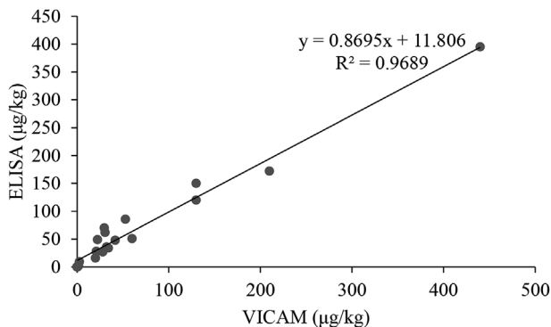
Fig. 2. Correlation between aflatoxin B 1 (AFB 1 ) levels obtained using VICAM and ELISA analytical methods. Analysis was done in a subset of 20 randomly selected samples of the maize collected at preharvest.
