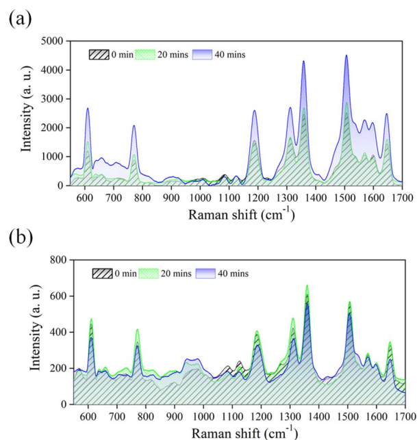
Fig. 4 Raman spectra of R6G ( 10^{-3} M) for PSi substrates exposed to UV irradiation for different durations and fabricated (a) with and (b) without TiO 2 NPs in the precursor used in the PLIP process. All Raman spectra were obtained under the same conditions.
