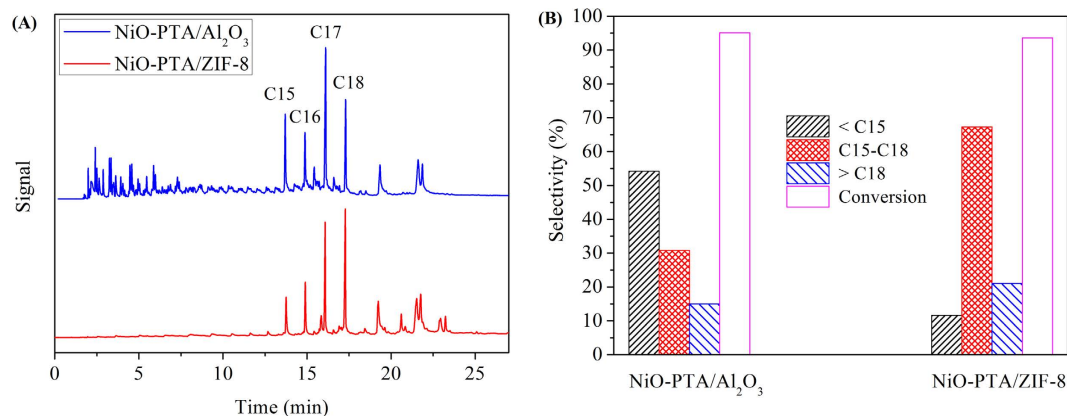
Figure 6. GC of products obtained from hydrocracking of Jatropha oil (A) and comparison to the selectivity of products and conversion of Jatropha oil (B) over the NiO-PTA/Al 2 O 3 and NiO-PTA/ZIF-8 catalyst (360 °C and 30 wt%PTA).
