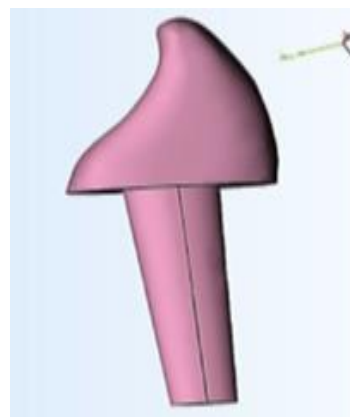
Fig. 2. Post and core model designed by Solid Work software
