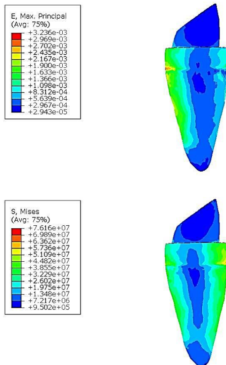
Fig. 10. Strain (A) and stress (B) at 2 and 5mm ferrule heights
