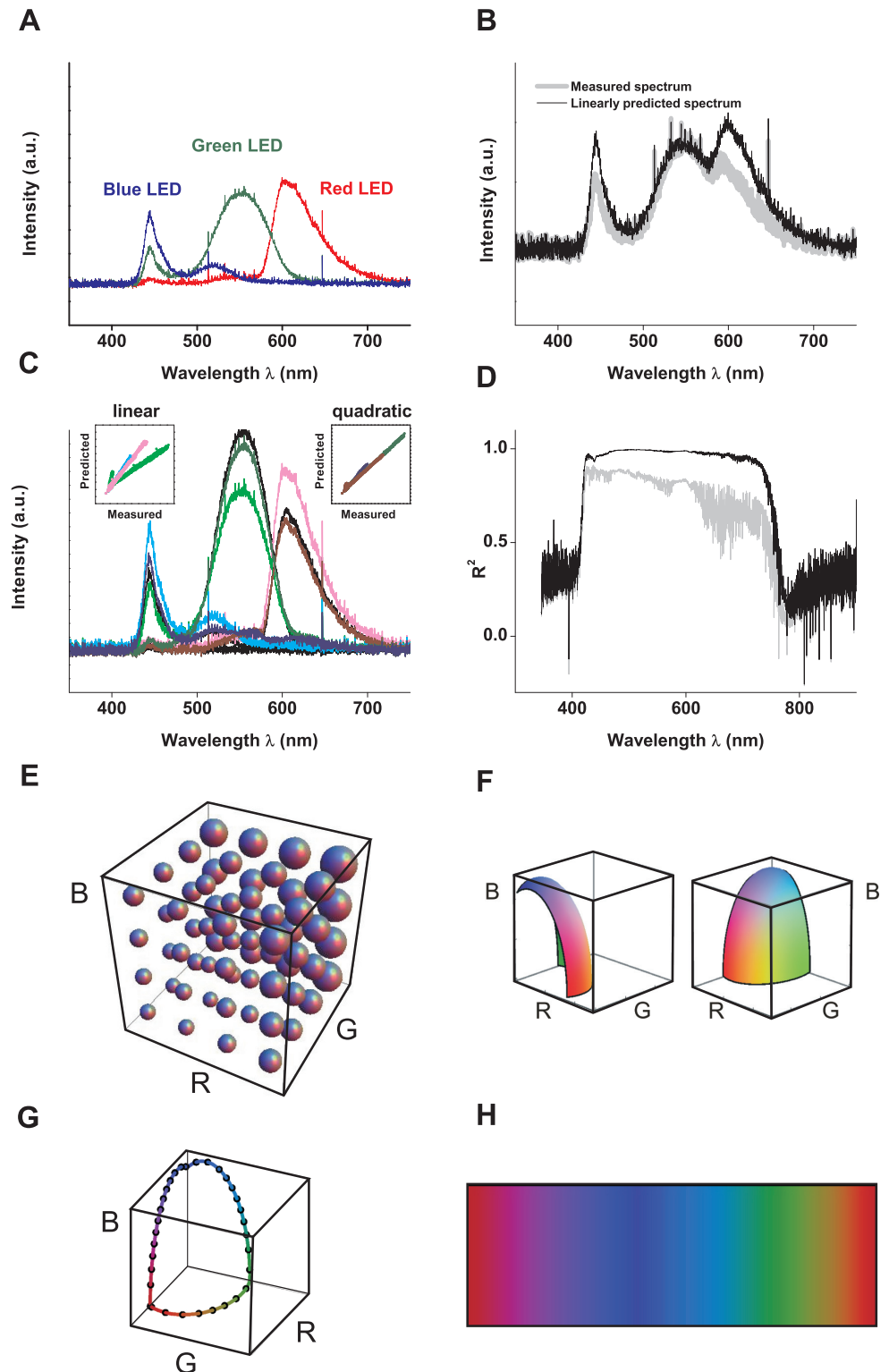
Fig 10. Calibration of the game. A: Spectra of the three LEDs of the computer screen, with coordinates (128, 0, 0) (red), (0, 128, 0) (green) and (0, 0, 128) (blue). B: Measured (gray) and linearly predicted (black) spectra, for a gray screen where RGB = (128, 128, 128) . C: Black curves: measured spectra for RGB = (255, 0, 0) , (0, 255, 0) and (0, 0, 255) . Light colors (pink, light green and cyan): spectra predicted with the linear model. Dark colors (red, green, blue): predictions for the quadratic model. Inset: comparison between predicted and measured intensities for the two
