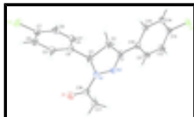
Fig. 1. Molecular structure of (I), C_{17}H_{14}Cl_2N_2O , showing the atom labeling scheme and 50% probability displacement ellipsoids.
