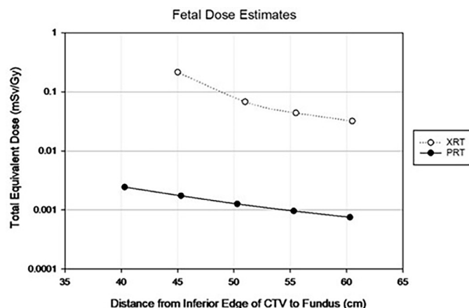
Figure 3 Measured total equivalent dose in millisieverts per prescription gray as a function of distance from the inferior edge of the CTV in centimeters cm to the center of the detector (fundus) from the PRT and XRT brain plan. Abbreviations: CTV = clinical target volume; PRT = proton therapy; XRT = x-ray radiation therapy.
