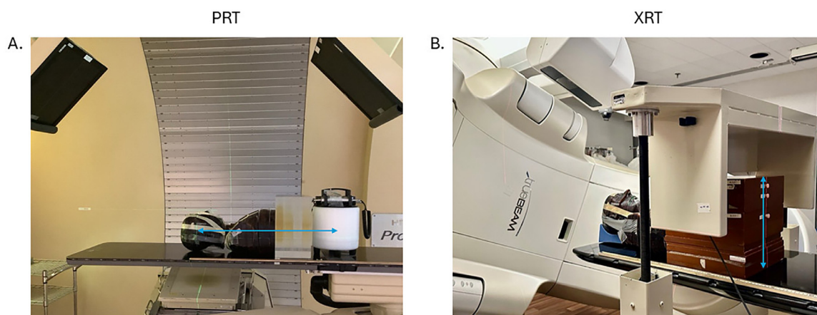
Figure 2 (A) PRT setup for fetal dose measurements using a WENDI-2 meter, anthropomorphic phantom, and acrylic. The arrow represents the isocenter to fundus distance. (B) XRT setup with an ion chamber, anthropomorphic phantom, solid water block, and fetal shield. The arrow represents the anterior-to-posterior patient thickness at the fundus.
