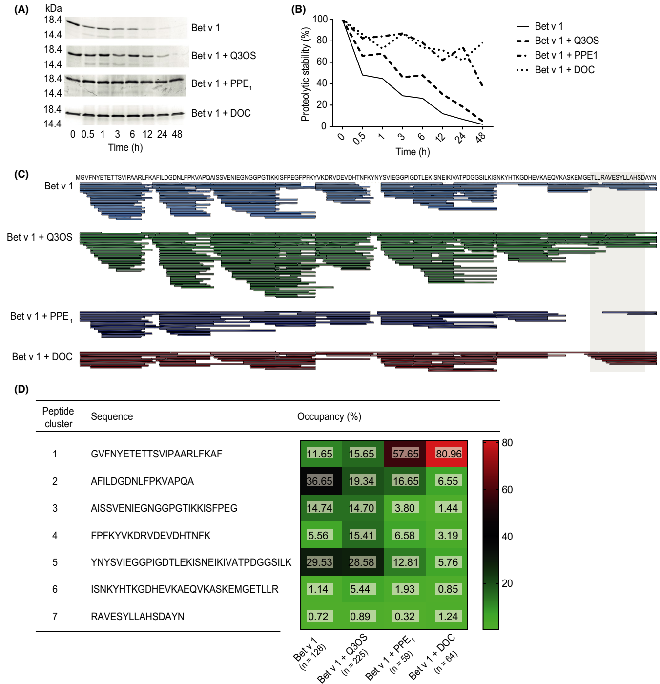
FIGURE 1 Ligand interaction alters the proteolytic susceptibility of Bet v _1. A, SDS-PAGE analysis of in vitro endolysosomal degradation of Bet v _1 with and without ligand recorded at different time points from 0 to 48 h and B, densitometric analysis thereof, interpreted with Image Lab 4.0.1 Software (Bio-Rad). C, Generated peptide clusters obtained after 12 h of proteolytic degradation analyzed by mass spectrometry. D, The peptide sequences were grouped into seven degradation clusters with their relative abundance, as derived from MS intensities. The number of unique peptide sequences is shown in brackets
