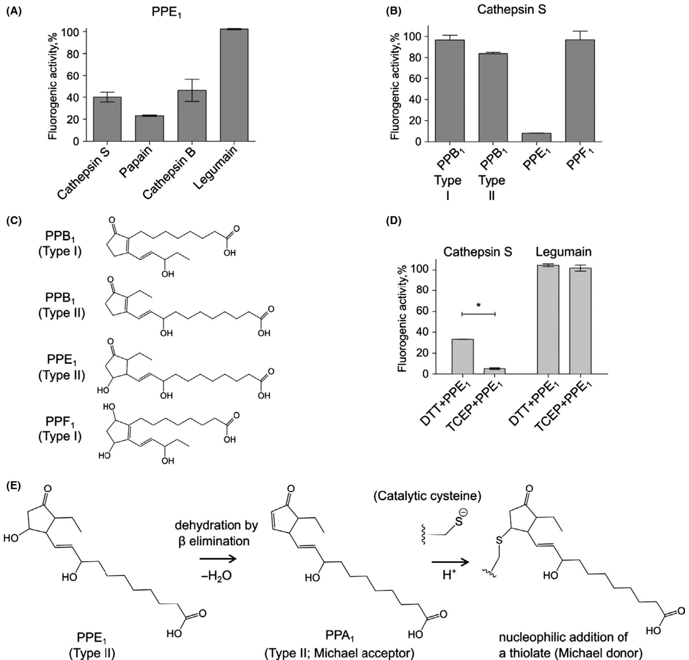
FIGURE 4 Inhibition mechanism of PPE 1 . A, PPE 1 inhibits papain-like cysteine proteases, but not legumain. Papain-like cysteine proteases (rat cathepsin B, cathepsin S, and papain) and legumain were incubated with PPE 1 (5 \mu\text{mol/L} ), and fluorogenic activities were recorded after 15 min. B, Effect of phytohormones (0.1 mmol/L) structurally related to PPE 1 on cathepsin S activity. Fluorogenic activity was recorded after 15 min. C, Chemical structure of phytohormones used in (B). D, Effect of reducing agents on PPE 1 inhibition of cathepsin S and legumain. The ability of proteases to cleave the fluorogenic substrates with and without PPE 1 (5 \mu\text{mol/L} ) in the presence of DTT and TCEP. Fluorogenic substrates used for cathepsin S and legumain were Z-VVR-AMC and Z-AAN-AMC, respectively. Error bars indicate standard deviations. Asterisk indicates statistical significance with P < 0.05 . E, Proposed mechanism of cathepsin S inhibition by PPE 1 . PPE 1 undergoes spontaneous dehydration by \beta -elimination, resulting in PPA 1 . 43 This reaction does not occur with PPB 1 , which lacks a hydroxyl group in the ring, and is disfavored in PPF 1 due to the missing ketone group. The resulting PPA 1 is an electrophile (Michael acceptor) and can be readily attacked by the nucleophilic cysteine of cathepsin S (Michael donor) at the \beta carbon to form a covalent adduct, 48 thus inhibiting cathepsin S activity
