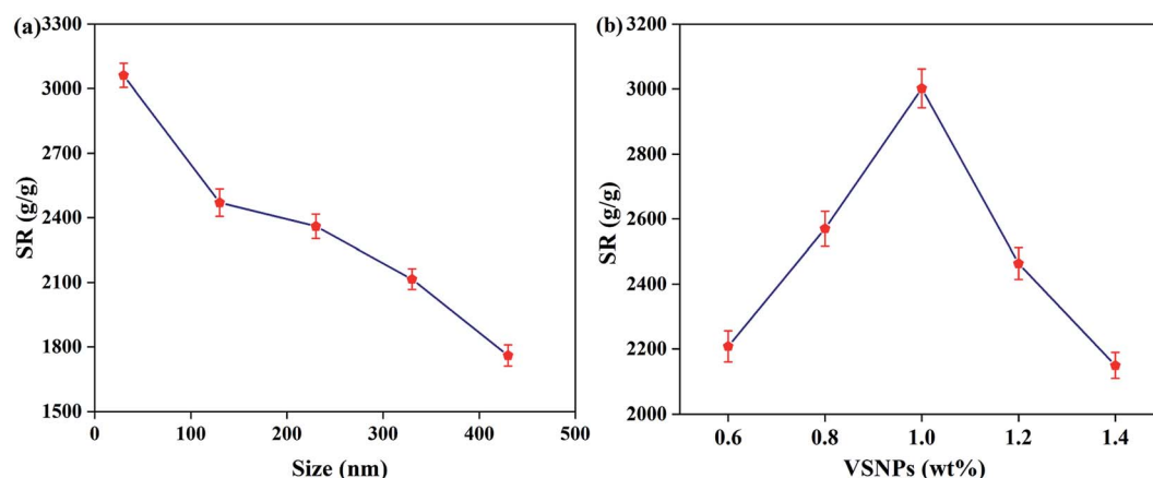
Fig. 2 (a) SR of the PAA NC hydrogel with different sizes and (b) the concentration of the VSNNPs in pure water at 303 K.
