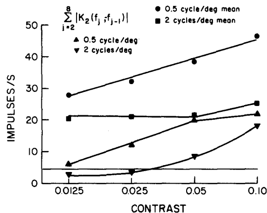
FIGURE 9. Elevation of mean rate with contrast. The mean rate of an on-center Y cell is plotted as a function of contrast. The results from two different experimental runs at two different spatial frequencies are shown: those for 0.5 cycle/deg (●) and 2 cycles/deg (■). The 0.5 cycle/deg grating was placed at the null position for first-order responses. At 2 cycles/deg there were no first-order responses, only second-order responses. Also plotted in the figure are the sums
