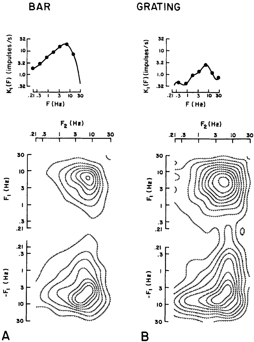
A B FIGURE 3. Comparison of responses of an on-center Y cell to a bar and a grating. (A) The stimulus was a 1.0^\circ \times 20^\circ vertical bar, positioned over the receptive-field center. (B) The stimulus was an 0.6 cycle/deg grating, positioned near the null spatial phase for the first-order response. The contrast modulation signal was a sum of eight sinusoids, each producing a contrast of 0.05. Although the maximum first-order response varied from 17 impulses/s (bar) to 3 impulses/s (grating), the second-order responses were virtually identical. Unit 13/10.
