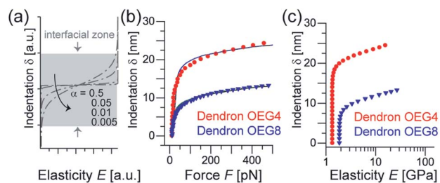
Fig. 3 (a) Elasticity profile of an interfacial zone between two phases possessing different levels of elasticity (eqn (2)). Decrease in transition parameter \alpha results in slower transition. (b) Indentation–force relationships for dendron OEG4 (red symbols) and dendron OEG8 (blue symbols) with the best fit results (solid lines). (c) Dependence of Young's modulus of two dendrons as a function of indentation depth. The apparent film elasticity values were determined from the regions where Young's modulus is independent from indentation depth. Interface model.
