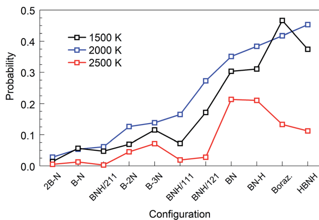
Fig. 2 Parameters of the synthesis quality (PSQs) for all initial configurations and selected temperatures at t = 1 ns. Precursor subgroup species are ordered along the abscissa following the increasing order of PSQ at 2000 K.
