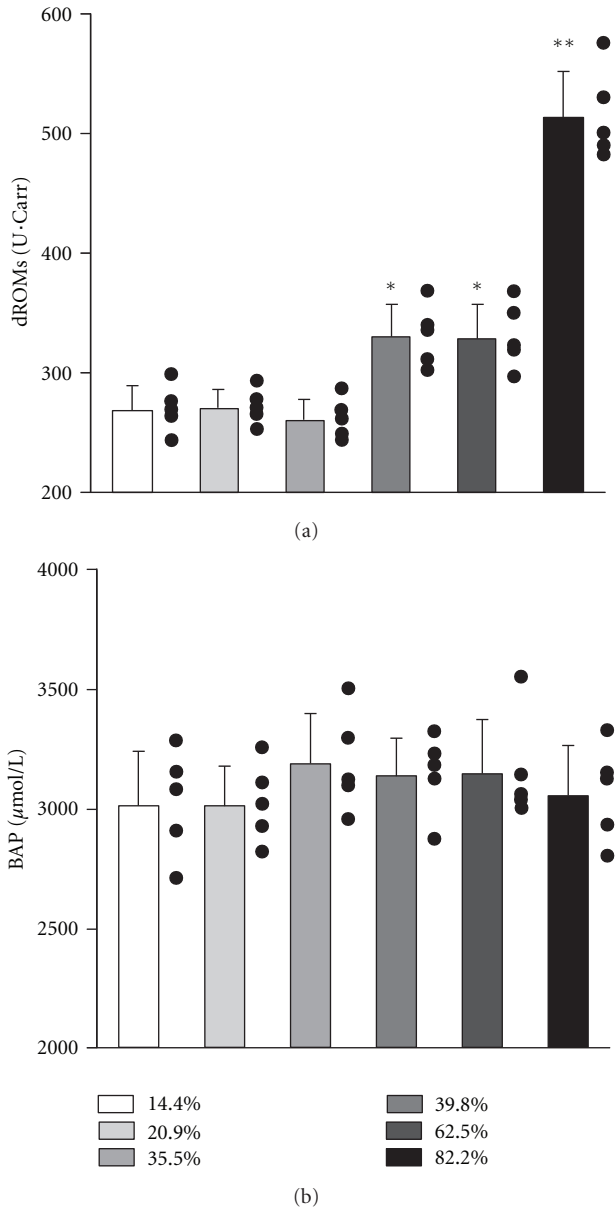
FIGURE 1: Levels of derivatives of reactive oxygen metabolites (a) and biochemical antioxidant potential (b) of rats after exposure to different concentrations of oxygen for 24 h. Values are expressed as the mean and standard deviation ( n = 5 for each group). Five dots on the right side of the bar are the individual values of rats in each group. dROMs: derivatives of reactive oxygen metabolites; BAP: biochemical antioxidant potential. * P < 0.05 compared with values of 14.4%, 20.9%, and 35.5% oxygen; ** P < 0.05 compared with values of 14.4%, 20.9%, 35.5%, 39.8%, and 62.5% oxygen.
