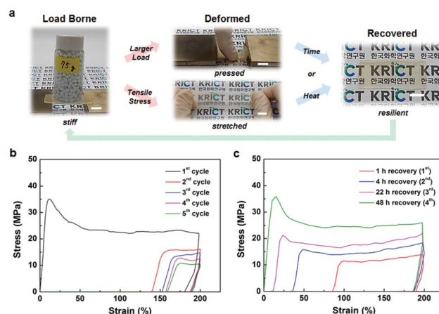
Fig. 2 Stiff, strong, tough, and resilient properties of BMPN8. (a) Photographs of load borne, deformed, and recovered BMPN8 (scare bar = 1 cm). (b) Cyclic stress–strain curves of pristine BMPN8. (c) Cyclic stress–strain curves of the pre-stretched BMPN8 (in (b)) after recovered for 1, 4, 22, and 48 h at 25 °C. The cyclic tensile testing was performed at strain rate and limit of 0.0067 s -1 and 200%, respectively.
