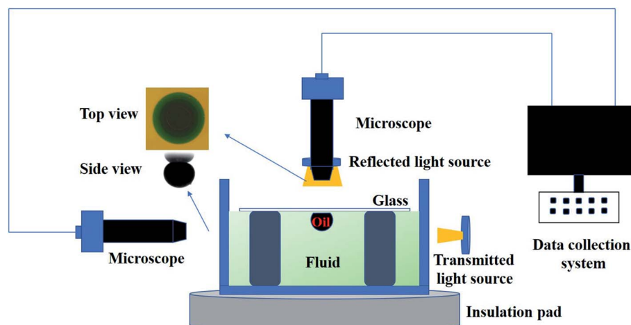
Fig. 2 Crude oil removal experiment device.
