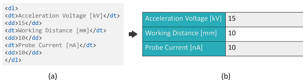
Figure 5. HTML description list rendering in eLabFTW. (a) Title-value pairs in the HTML description list format, and (b) the rendered description list with a custom CSS styling. CSS, Cascading Style Sheets.
