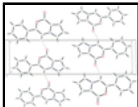
Fig. 2. The crystal packing of the title compound viewed along the b axis. Intermolecular C—H...O interactions are drawn as dashed lines.
