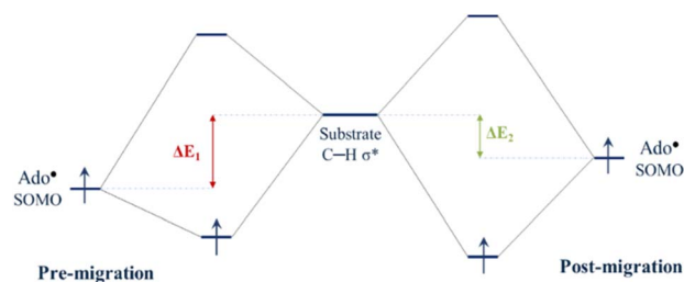
Fig. 5 Simple MO energy diagram illustrating the interaction between the Ado • SOMO in pre-migration and post-migration models and the substrate C–H \sigma^* . Because the energy gap ( \Delta E ) between Ado • SOMO and C–H \sigma^* is smaller in Post models compared to Pre models ( \Delta E_1 > \Delta E_2 ), these two MOs can interact with each other more efficiently in Post models. The more favorable interaction in the Post model compared to Pre results in the reactivity difference observed between the two.
