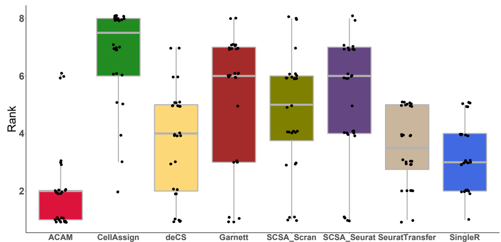
Figure 3. Rank of the compared methods. Boxplot of the rank of each method according to four evaluation metrics: accuracy, balanced accuracy, macro F1-score, and MCC on seven datasets is shown. A lower rank represents better performance (one is the best and eight is the worst).
