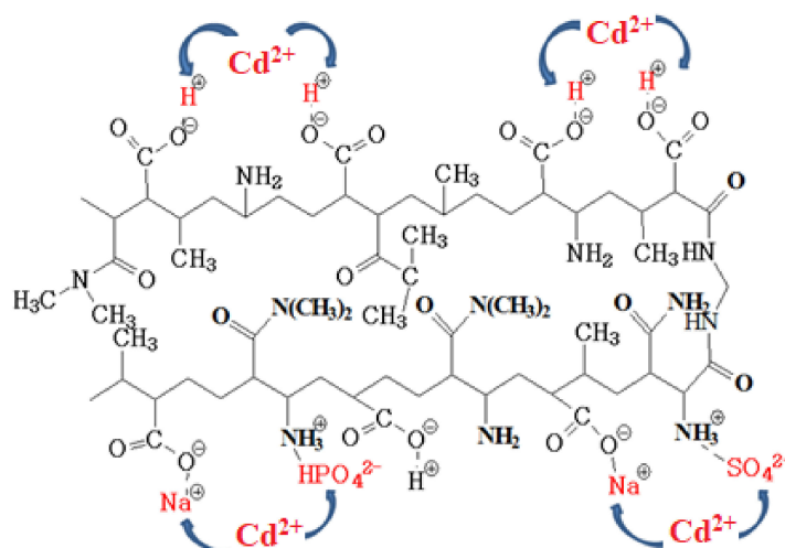
Figure 9. Proposed complexation of Cd 2+ with functional groups of p(MAAc)-DMAAm-AA.
