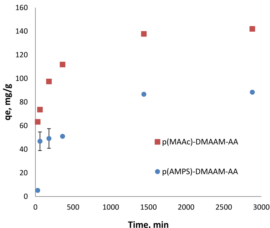
Figure 3. Cd 2+ removal kinetics on the p(MAAc)-DMAAM-AA and p(AMPS)-DMAAM-AA cryogels (70 mg of cryogel in 100 mL of solution) at pH 5.5.
