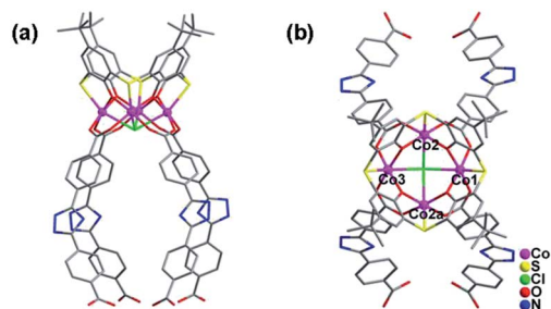
Fig. 1 Coordination of the \text{Co}_4 -TC4A SBU in CIAC-236. (a) Side view and (b) top view. Symmetry codes: a: x, 1.5 - y, z .
