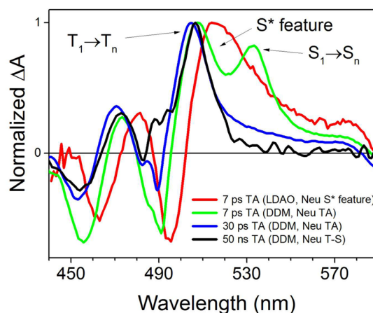
Figure 4. Comparison of transient absorption spectra taken for both LH2 batches (LDAO and DDM preps) at time delays at which the main S_1 \rightarrow S_n ESA of neurosporene decayed. For the LDAO-Tris-LH2, the TA spectrum taken at 7 ps corresponds to S^* spectral feature. For comparison, also TA spectrum of the DDM-HEP-LH2 at the same delay time is shown. The 30 ps spectrum (free of S_1 \rightarrow S_n ESA band) is identical to the triplet–minus–singlet (T–S) spectrum of neurosporene taken at 50 ns after excitation. All spectra were normalized to unity at their maxima.
