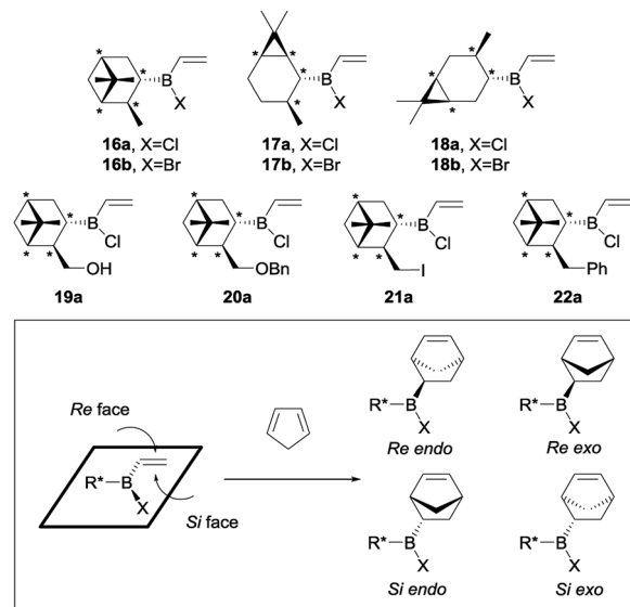
Scheme 5 Diels–Alder reactions of chiral alkylhalovinylboranes 16–22 with cyclopentadiene.
