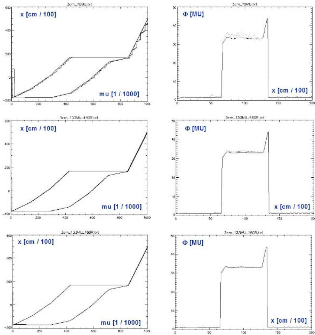
FIG. 5. The same quantities as in Fig. 2 but obtained for various combinations (R \text{ [MU/min]}, MU_{\text{tot}} \text{ [MU]}) = (800, 70) , (480, 133) , (160, 133) . MU_{\text{tot}} = 133 is the original number of monitor units calculated by the IMRT system. When the dose rate is decreased, the maximum opening artifact and the local wiggles in the MLC trajectory are decreased.
