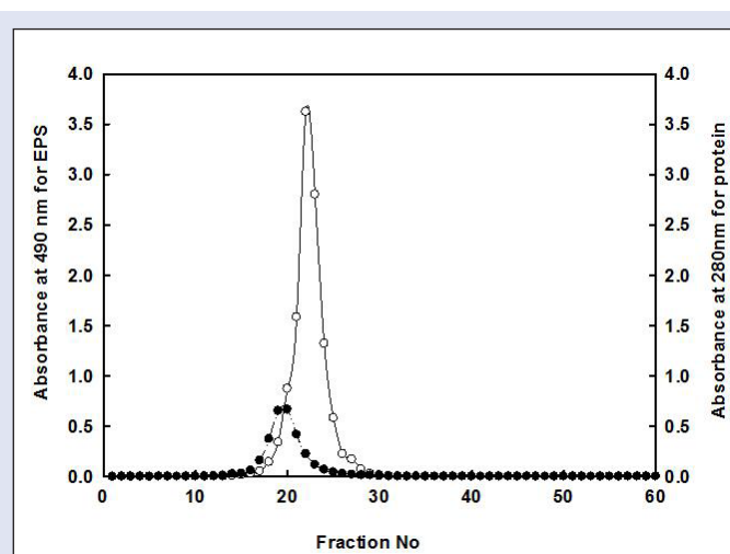
Figure 3: Elution profiles of the EPS in Sepharose CL-6B chromatography. Eluate was analyzed by measuring the absorbance at 490 nm for carbohydrate (o) and the absorbance at 280 nm for protein (●).
