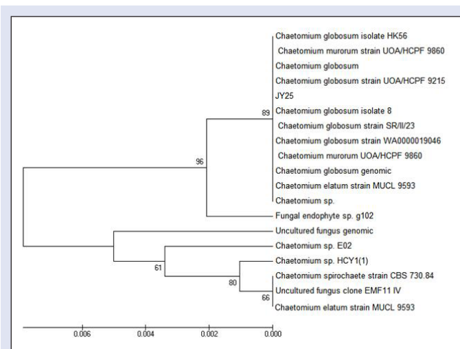
Figure 2: The phylogenetic dendrogram for Chaetomium sp. JY25 and related strains based on the ITS rDNA sequence. Numbers in parentheses are accession numbers of published sequences. Bootstrap values were based on 1000 replicates.
