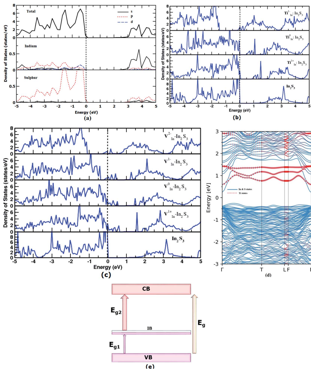
Fig. 3 Density of states of (a) pure \gamma - \text{In}_2\text{S}_3 (b) \text{Ti}_{\text{In}}^0 - \text{In}_2\text{S}_3 , and (c) \text{V}_{\text{In}} - \text{In}_2\text{S}_3 . (d) Electronic band structure of \text{Ti}_{\text{In}}^0 - \text{In}_2\text{S}_3 and (e) illustration of the possible multi-transitions in an intermediate band semiconductor.
