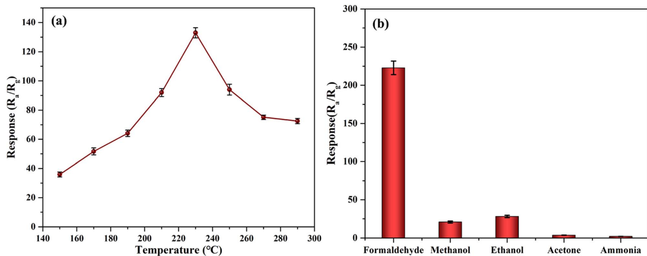
Fig. 5 The response ( R_a/R_g ) of sensors based on mesoporous nanoparticles. (a) Temperature-dependent sensing responses to 100 ppm HCHO. (b) Selectivity of the sensor to four kinds of interfering gases.
