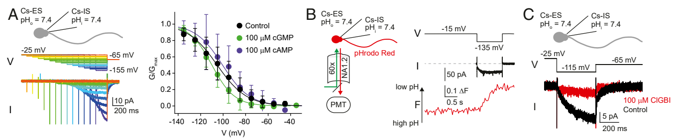
Fig. 5. HCNL1 acidifies zebrafish sperm upon hyperpolarization. (A, Left) Whole-cell patch clamp recording of hyperpolarization-activated currents in zebrafish sperm in the presence of Cs + to block CNGK. (A, Right) GVs derived from tail currents with or without 100 \mu\text{M} cAMP or cGMP in the intracellular solution. Error bars denote SD. (B) Whole-sperm patch clamp fluorimetry recording with the fluorescent pH indicator pHrodo Red. (C) Block of hyperpolarization-activated current in zebrafish sperm by 100 \mu\text{M} CIGBI ( 73 \pm 9\% , n = 4 ). Error bars denote SD.
