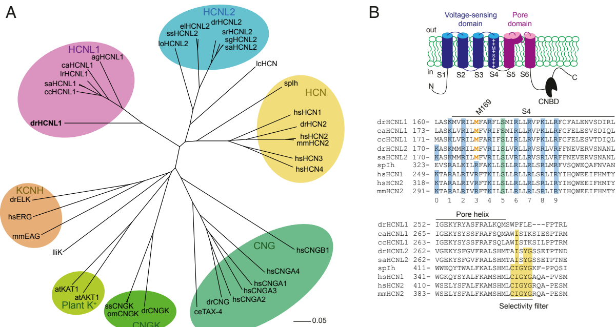
Fig. 2. Structural features of the zebrafish HCNL1 channel. (A) Phylogenetic tree of ion channels containing a CNBD (accession numbers of HCNL1/2 channels are listed in SI Appendix, Table S1 ). The scale bar represents 0.05 substitutions per site. (B, Top) Cartoon of HCNL1. (B, Bottom) Alignment of S4 transmembrane helices and pore domains of the HCNL1/2 and HCN channels.
