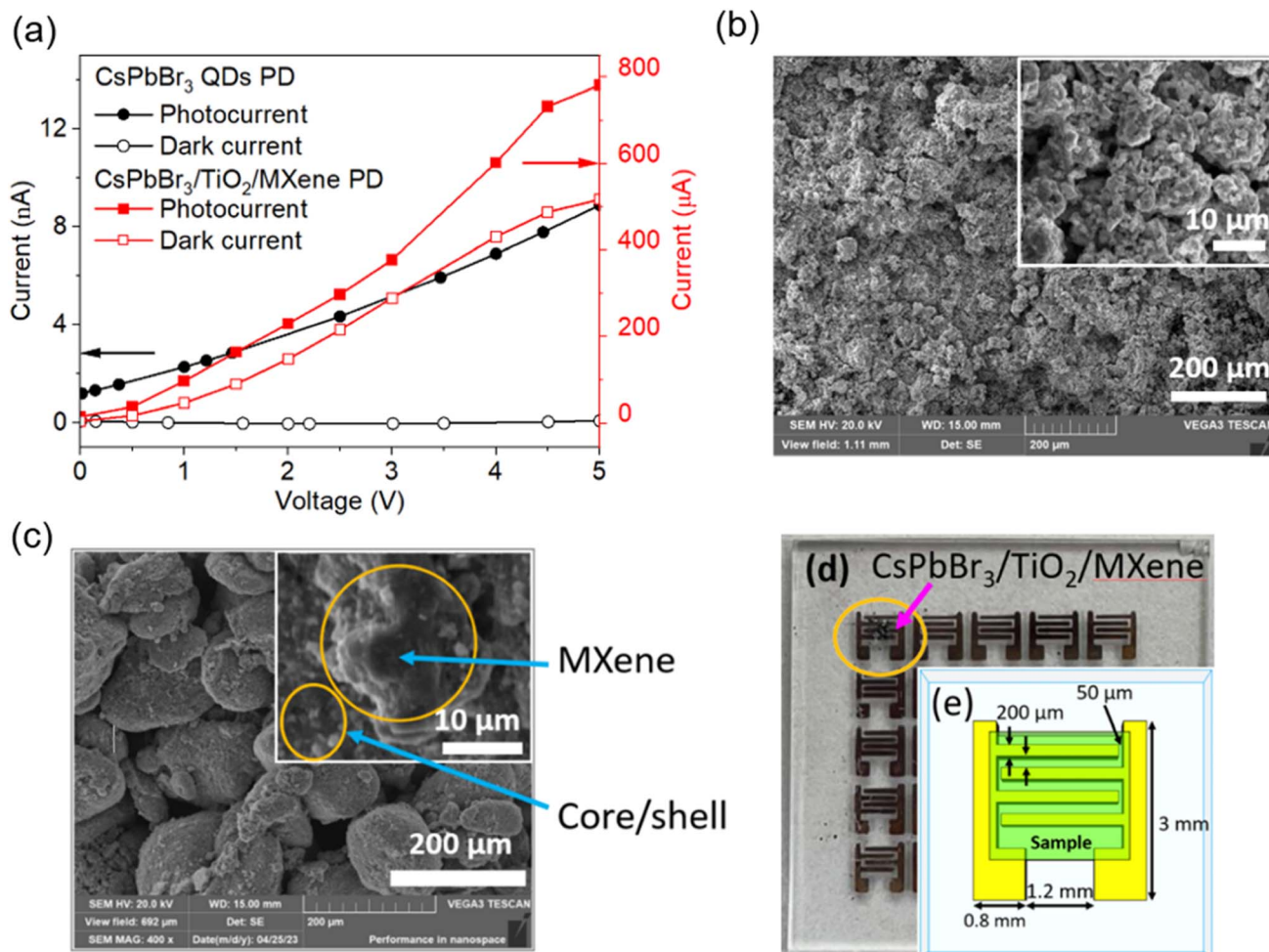
Fig. 4 (a) I-V curve of the CsPbBr 3 QD PD and CsPbBr 3 /TiO 2 /MXene PD in the dark and under illumination of a blue laser, SEM images of the (b) CsPbBr 3 /TiO 2 PD and (c) CsPbBr 3 /TiO 2 /MXene PD, (d) optical image of the CsPbBr 3 /TiO 2 /MXene PD and (e) schematic 2D view of the measurements of Au interdigitated electrodes with the sample.
