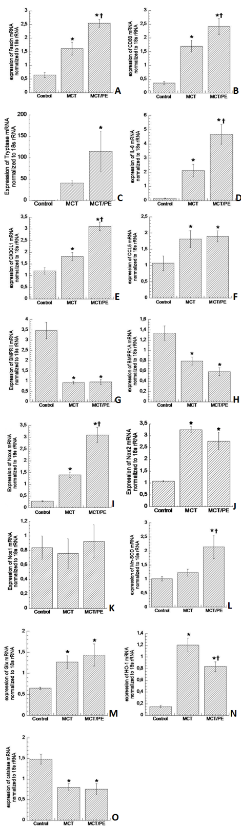
Figure 3 mRNA gene expression measured by real-time PCR. 18s rRNA was used as an internal housekeeping control. Results are provided as arbitrary units. A: Fascin. B: CD68. C: tryptase. D:
