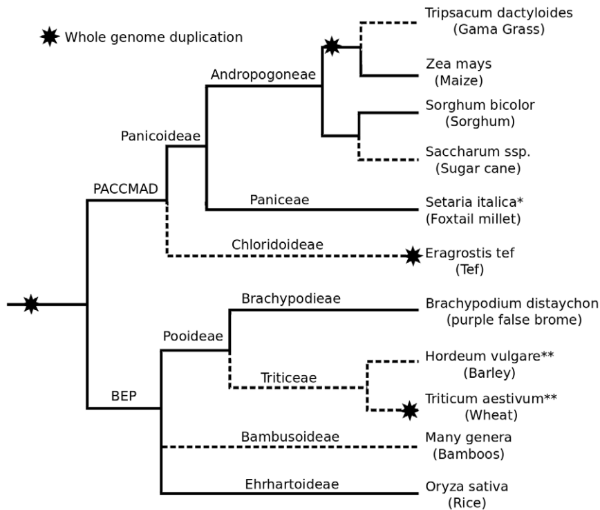
Figure 1. Phylogenetic relationships of notable and sequenced grass species. Branch lengths not to scale. *The genome sequencing of foxtail millet by the joint genome institute is complete, but has not yet been published. Therefore it is not included in our analyses (SI 1). **Projects to sequence the genomes of barley and wheat are announced or in progress. doi:10.1371/journal.pone.0017855.g001
