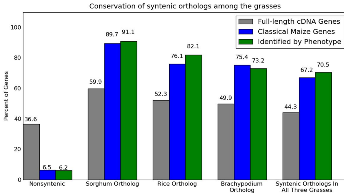
Figure 3. Syntenic conservation of the classical maize genes in other grasses. Comparison of the proportion of genes identified by a mutant phenotype prior to cloning (N=111), all classical maize genes (N=464), and all maize genes supported by full length cDNA evidence (N=34579) for which syntenic orthologs could be identified in the other three grass species with sequenced genomes: sorghum, rice, and brachypodium.
