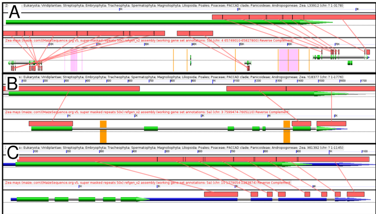
Figure 2. Examples of manually identified errors in maize gene annotations. Graphics from GEvo comparative sequence alignment tool. Annotated cDNAs from GenBank are compared to regions of the maize B73_refgen2 genome. Features on the forward strand are displayed above the dotted line, and features on the reverse strand are displayed below the line. Grey lines mark the extent of gene models with CDS sequences in green and UTR sequences in blue. Orange bars mark the gaps between assembled contigs of the maize genome (stretches of N's). Red boxes connected by lines show sequences identified as homologous by blastn. A. A comparison of the coding sequence of aspartate kinase-homoserine dehydrogenase1 to the region of maize chromosome 4 that contains the three gene models –from left to right, GRMZM2G365423, GRMZM2G389303, and GRMZM2G437977 – among which the exons of this gene have been divided. An interactive version of this graphic can be regenerated in GEvo using the following link: http://genomeevolution.org/r/25xh B. A comparison of cytokinin oxidase1 to GRMZM2G146644, a gene model which includes the 5' and 3' ends of cko1 but has also incorporated unrelated exons from another maize genome contig. Regenerate analysis: http://genomeevolution.org/r/25s5 C. The coding sequence of ferredoxin homeolog2 which maps to a region of the maize genome annotated as the 3' UTR of GRMZM2G147266. Regenerate analysis: http://genomeevolution.org/r/25s7 . doi:10.1371/journal.pone.0017855.g002
