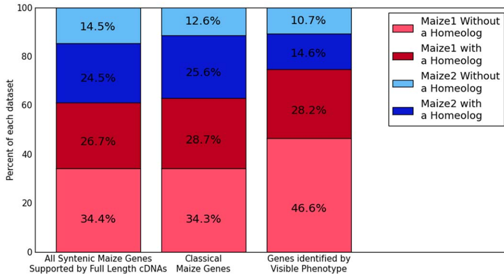
Figure 4. Distribution of classical maize genes between the two maize subgenomes. Comparison of the distribution of genes retained syntenically in at least one other grass species between the two subgenomes of maize as well as whether genes possess retained homeologs from the maize whole genome duplication. For syntenically retained maize genes with full length cDNA support N = 17956. For the subset of the classical maize gene list that are syntenically retained N = 429. For the subset of genes that were first identified by mutant phenotype and are syntenically retained N = 102.
