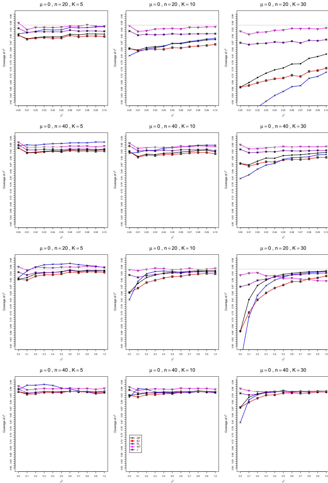
FIGURE 2 Mean difference: Coverage at the nominal 95% level of interval estimators of between-studies variance \tau^2 \in [0, 0.1] (top two rows) and \tau^2 \in [0, 1] (bottom two rows) for \mu = 0, q = 0.75 , when \sigma_C^2 = 1, \sigma_T^2 = 2, n = 20, 40 , and K = 5, 10, 30 . Light gray line at 0.95. BJ, Biggerstaff and Jackson; J, Jackson; PL, profile-likelihood; QP, Q-profile; WT, Welch-type [Colour figure can be viewed at wileyonlinelibrary.com ]
