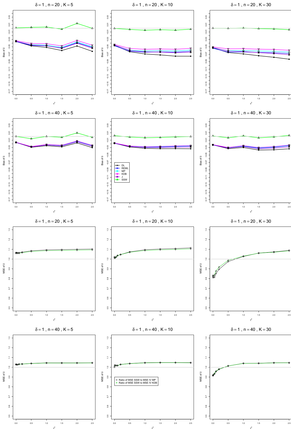
FIGURE 5 Standardized mean difference: Bias of the estimators of \delta and ratio of mean squared errors (MSEs) of SSW to inverse-variance-weighted estimators when \delta = 1, q = .5, n = 20, 40, and K = 5, 10, 30 . Light gray line at 0 for bias and at 1 for the ratio of MSEs. DL, DerSimonian-Laird; KDB, Kulinskaya-Dollinger-Bjørkestøl; J, Jackson; MP, Mandel-Paule; REML, restricted maximum-likelihood [Colour figure can be viewed at wileyonlinelibrary.com ]
