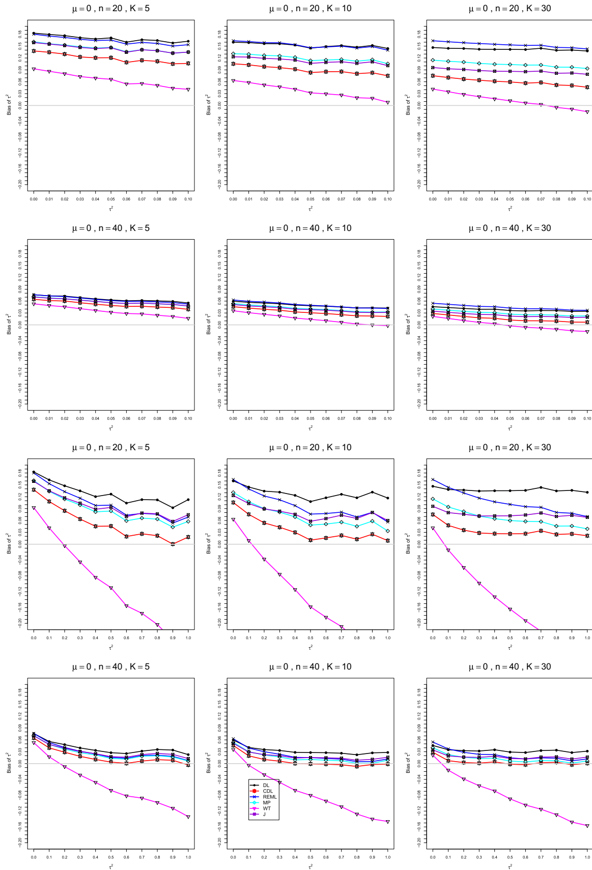
FIGURE 1 Mean difference: Bias of estimators of between-studies variance \tau^2 \in [0, 0.1] (top two rows) and \tau^2 \in [0, 1] (bottom two rows) for \mu = 0, q = 0.75 when \sigma_C^2 = 1, \sigma_T^2 = 2, n = 20, 40, and K = 5, 10, 30 . Light gray line at 0. CDL, corrected DL; DL, DerSimonian-Laird; J, Jackson; MP, Mandel-Paule; REML, restricted maximum-likelihood; WT, Welch-type [Colour figure can be viewed at wileyonlinelibrary.com ]
