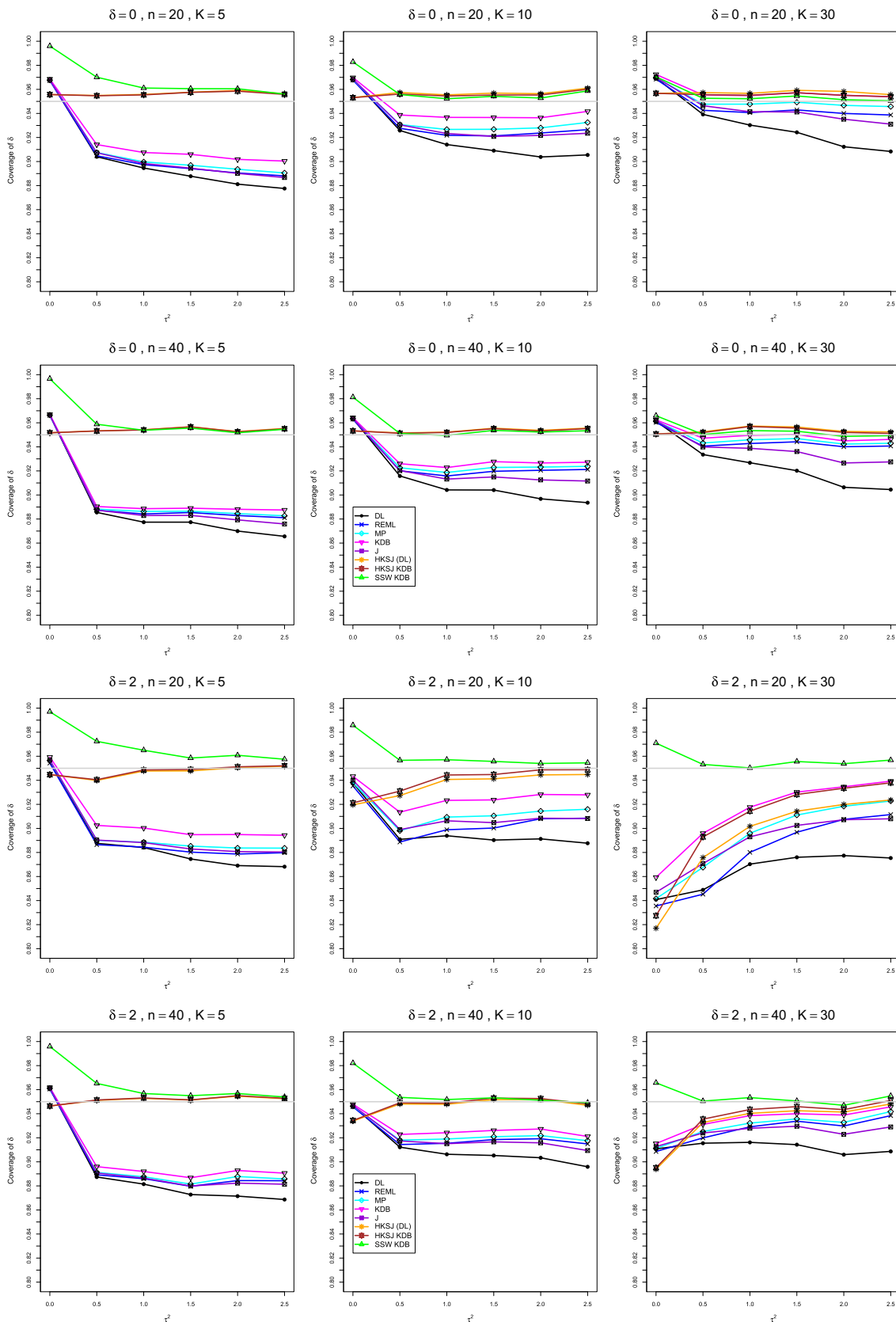
FIGURE 6 Standardized mean difference: Coverage of 95% confidence intervals for \delta when \delta = 0 (top two rows) and 2 (bottom two rows), q = .5 , n = 20, 40 , and K = 5, 10, 30 . Light gray line at 0.95. DL, DerSimonian-Laird; HKSJ, Hartung-Knapp-Sidik-Jonkman; J, Jackson; KDB, Kulinskaya-Dollinger-Bjørkestøl; MP, Mandel-Paule; REML, restricted maximum-likelihood [Colour figure can be viewed at wileyonlinelibrary.com ]
