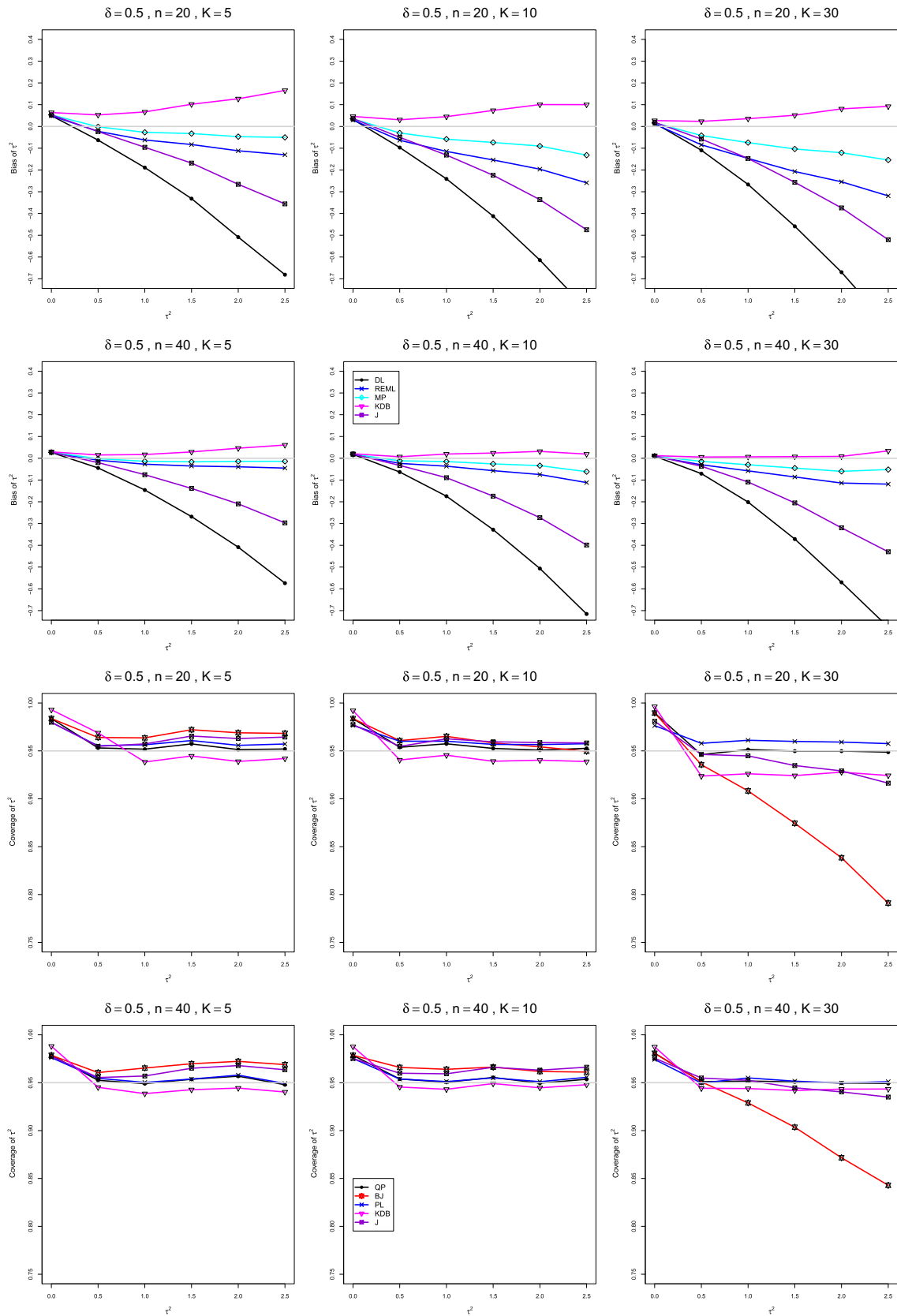
FIGURE 4 Standardized mean difference: Bias and coverage at nominal 95% level in estimation of between-studies variance \tau^2 for \delta = 0.5 , q = .5 , n = 20, 40 , and K = 5, 10, 30 . Light gray line at 0 for bias and at 0.95 for coverage. BJ, Biggerstaff and Jackson; DL, DerSimonian-Laird; KDB, Kulinskaya-Dollinger-Bjørkestøl; J, Jackson; MP, Mandel-Paule; PL, profile-likelihood; QP, Q-profile; REML, restricted maximum-likelihood [Colour figure can be viewed at wileyonlinelibrary.com ]
