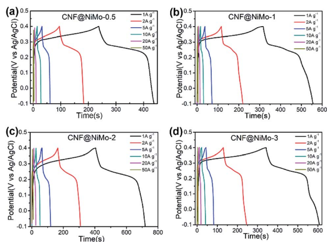
Fig. 5 Galvanostatic charge/discharge voltage profiles of (a) CNF@NiMo-0.5, (b) CNF@NiMo-1, (c) CNF@NiMo-2, and (d) CNF@NiMo-3 electrodes in the voltage range of -0.1 – 0.4 \text{ V vs. Ag/AgCl} .
