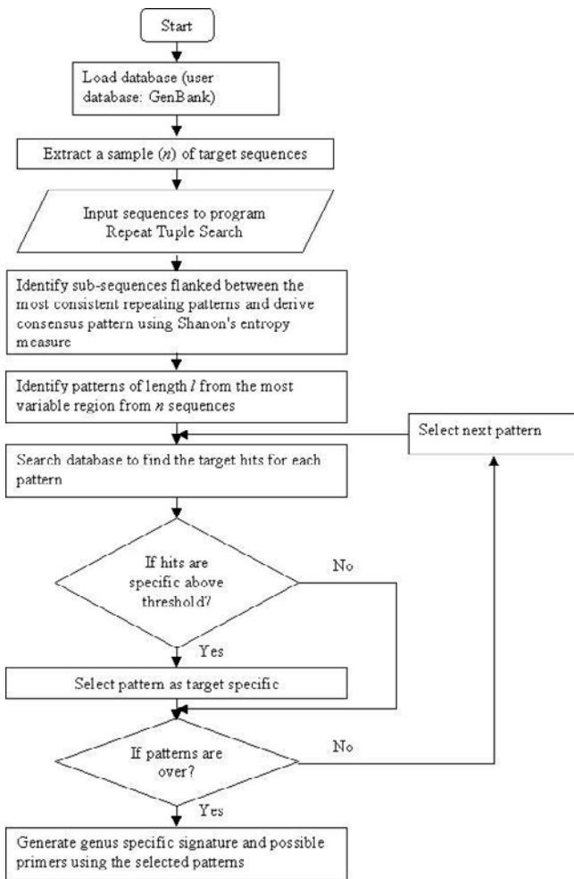
Figure 1 Flow chart summarizing the procedure for identifying target specific patterns
