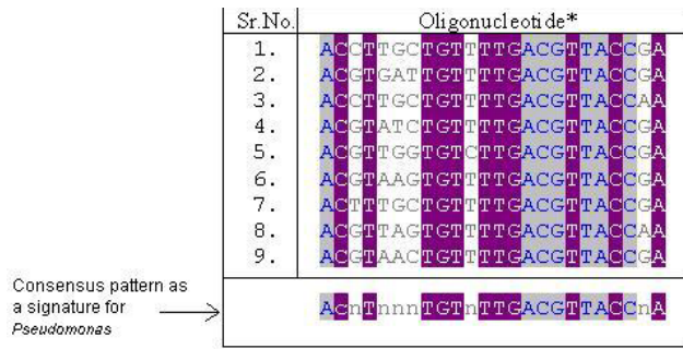
Figure 5 Patterns showing nearly 70% specificity to genus Pseudomonas and a consensus pattern as a signature for Pseudomonas .
