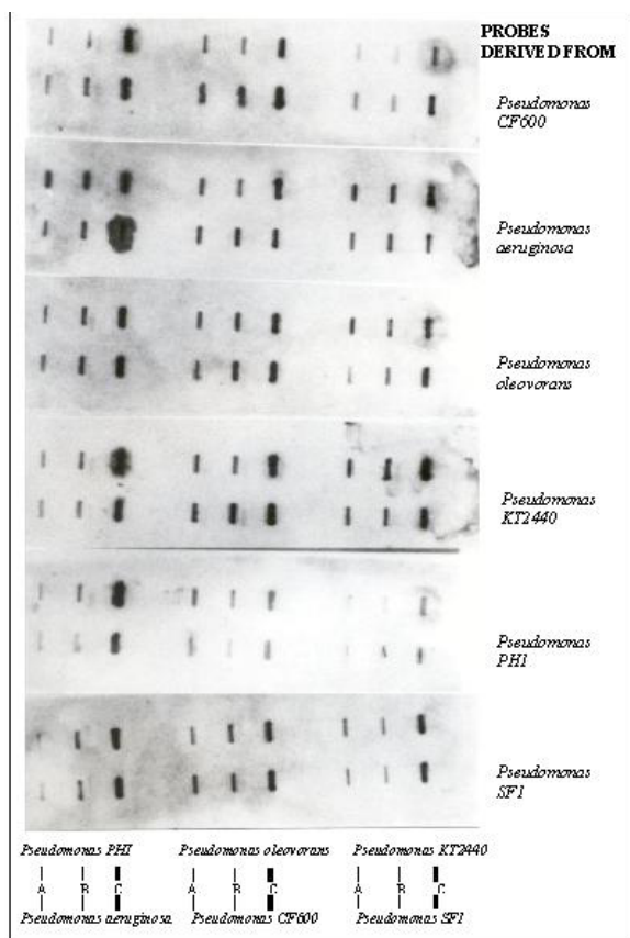
Figure 8 Demonstration of specificity of PCR amplified product for genus Pseudomonas by Slot-Blot hybridization data. PCR product was generated using signature primer as shown in Figure 7. Biotinylated probes were generated from PCR amplified 150 bp products using the BioPrime DNA Labeling Kit, Gibco BRL, USA. Six probes were derived using six different Pseudomonas strains as mentioned on the right panel of the figure. The same six strains were used as templates in the hybridization as shown in the schematic representation at the bottom of the figure. Each probe was tested against all six strains. The cultures were grown overnight at 30°C and diluted to yield 1000, 5000 and 10,000 cells per 100 µl of sterile double distilled water. This was transferred to a nylon membrane using the Slot-Blot apparatus at positions A, B and C respectively, where A represents 1000 cells, B, 5000 cells and C represents 10,000 cells. The spotted membranes were immersed in SDS/BSA hybridization buffer (0.3 ml/cm 2 of membrane). Hybridization was carried out at 60°C in a hybridization oven, Amersham Pharmacia Biotech Ltd., UK. Hybridization signals were detected using the Photogene Nucleic Acid Detection System Version-2 (Gibco-BRL, USA), as per the manufacturer's instructions with high stringency washing. Chemiluminiscent signals were quenched on Kodak X-omat film after exposure of 30 min. The negative controls used were E. coli , Salmonella , Vibrio , Shigella and Staphylococcus as used in Figure 7 to show the specificity of probe. There were no hybridization signals observed in any of the negative controls (data not shown) even after overnight exposure.
