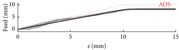
FIGURE 20: Comparison of the relationship between implant feed (y axis) and stylet extraction (x axis) for the AOS technique (red dotted line, strong linear relationship as recommended by the manufacturer) and for the optimized insertions (grey lines). The black line indicates an averaged profile for stylet extraction during the insertion process; even this small change appears to be advantageous compared with the conventional AOS technique.
