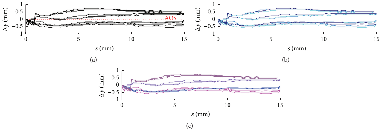
FIGURE 19: Process parameter \Delta y against stylet extraction s for all manually optimized insertions, normalized by the initial value at s = 0 mm. Refer to Figure 18 for legend.
