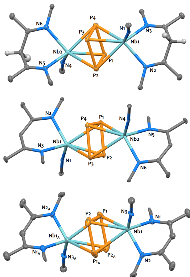
Figure 3. Solid-state molecular structures of 4 (top), 5 (middle), and 6 (bottom). Hydrogen atoms are not shown except for those of the methylene group of the protonated \text{BDI}^\# ligand in 4 , disopropyl aryl groups of the BDI ligands and \text{B}(\text{C}_6\text{F}_5)_4 counteranions have been removed, and ^t\text{Bu} moieties have been truncated for clarity. Niobium (light blue), phosphorus (orange), nitrogen (blue), hydrogen (white), and carbon (gray) atoms are represented with 50% probability ellipsoids. Selected metrical parameters are reported in Table 1.
