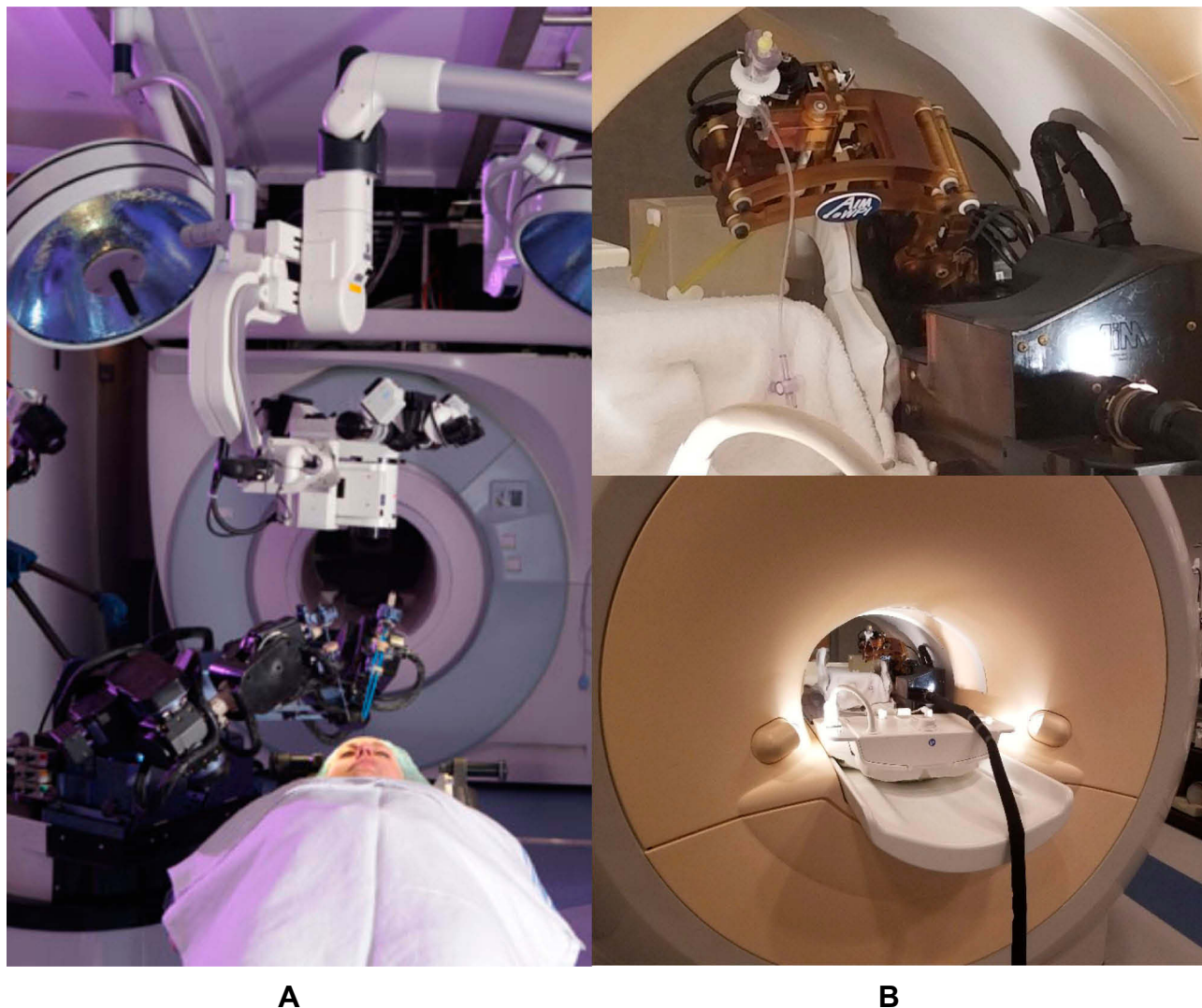
Figure 9 MRI-compatible neurosurgical robotics. (A) NeuroArm MRI-compatible neurosurgery robot, shown with patient in foreground and MRI scanner in the background. Reproduced with permission from NeuroArm. Project. 34 (B) Development of MRI-compatible deep brain stimulation robotic assistant by G.S. Fischer et al 35 Unpublished DBS robot images graciously contributed by G.S. Fischer of Worcester Polytechnic Institute.
