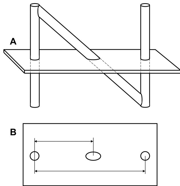
Figure 13 N-shaped fiducials for frame localization within a medical image. (A) Lateral view of the N-fiducial. Each N-fiducial result in a characteristic intersection with every image plane. (B) Typical intersection of the fiducial with a CT image. This intersection with the fiducial results in a pair of circles and an ellipse. The location of the ellipse between the two circles is a function of the height at which the tomographic image plane intersects the diagonal rod. Copyright © 2006. Wikipedia. Reproduced from uploader: Stereotactic surgery. Available from: https://en.wikipedia.org/wiki/Stereotactic_surgery . 66
