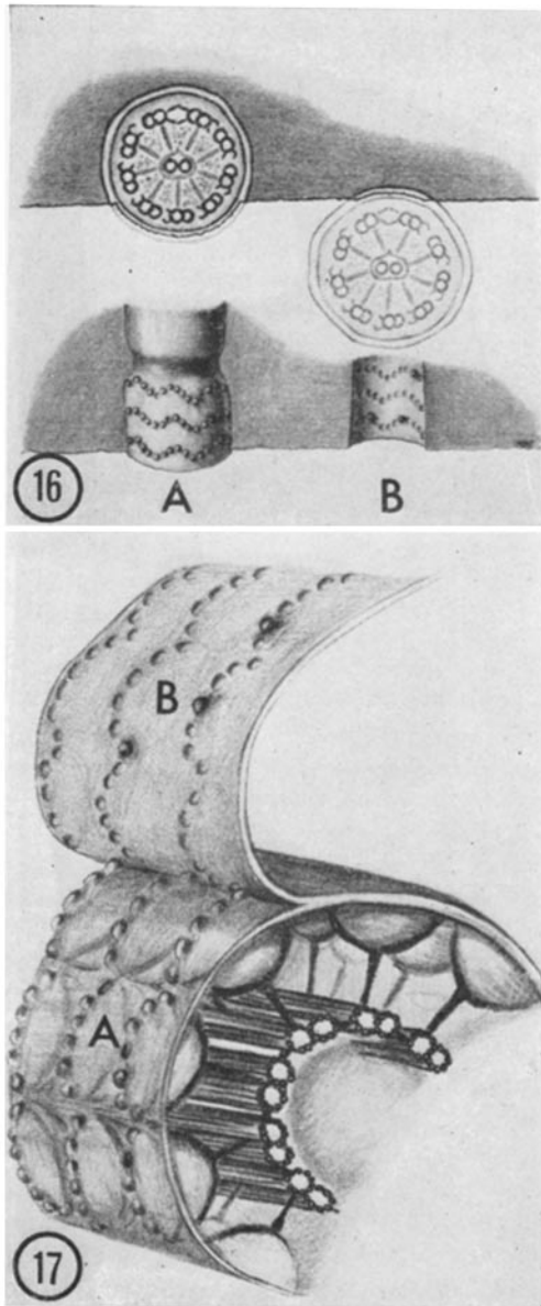
FIGURE 16 Schematic interpretation of the fracture process of the ciliary membrane necessary to produce the fracture faces of Figs. 7 and 8. The convex fracture face (A) is obtained when a portion of the membrane is torn away during the fracture process. Face A apposes the axoneme. The concave fracture face (B) apposes the exterior; the entire axoneme and a portion of the membrane is torn away during the fracture process.
