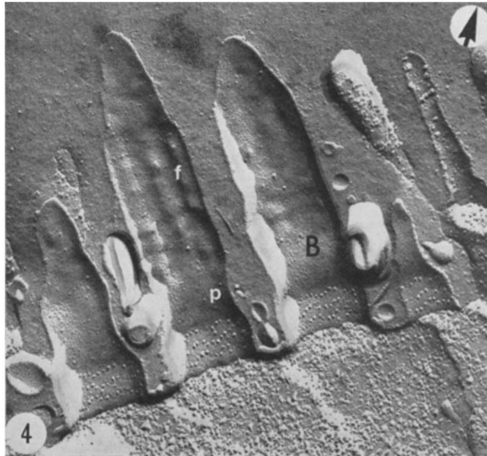
FIGURE 4 Freeze-fracture of the ciliated apical border of Elliptio gill lateral cell. The B (B) fracture faces of the ciliary membranes are exposed. The B faces contain fewer membrane-associated particles than the A faces (compare with Fig. 3). Above the basal plate (p), flutes (f) of the ciliary membrane are present. The basal plate region (p) is seen on the B face as a bulge that is devoid of particles. Below the basal plate, the B face aspect of the ciliary necklace is present. \times 67,500 .
