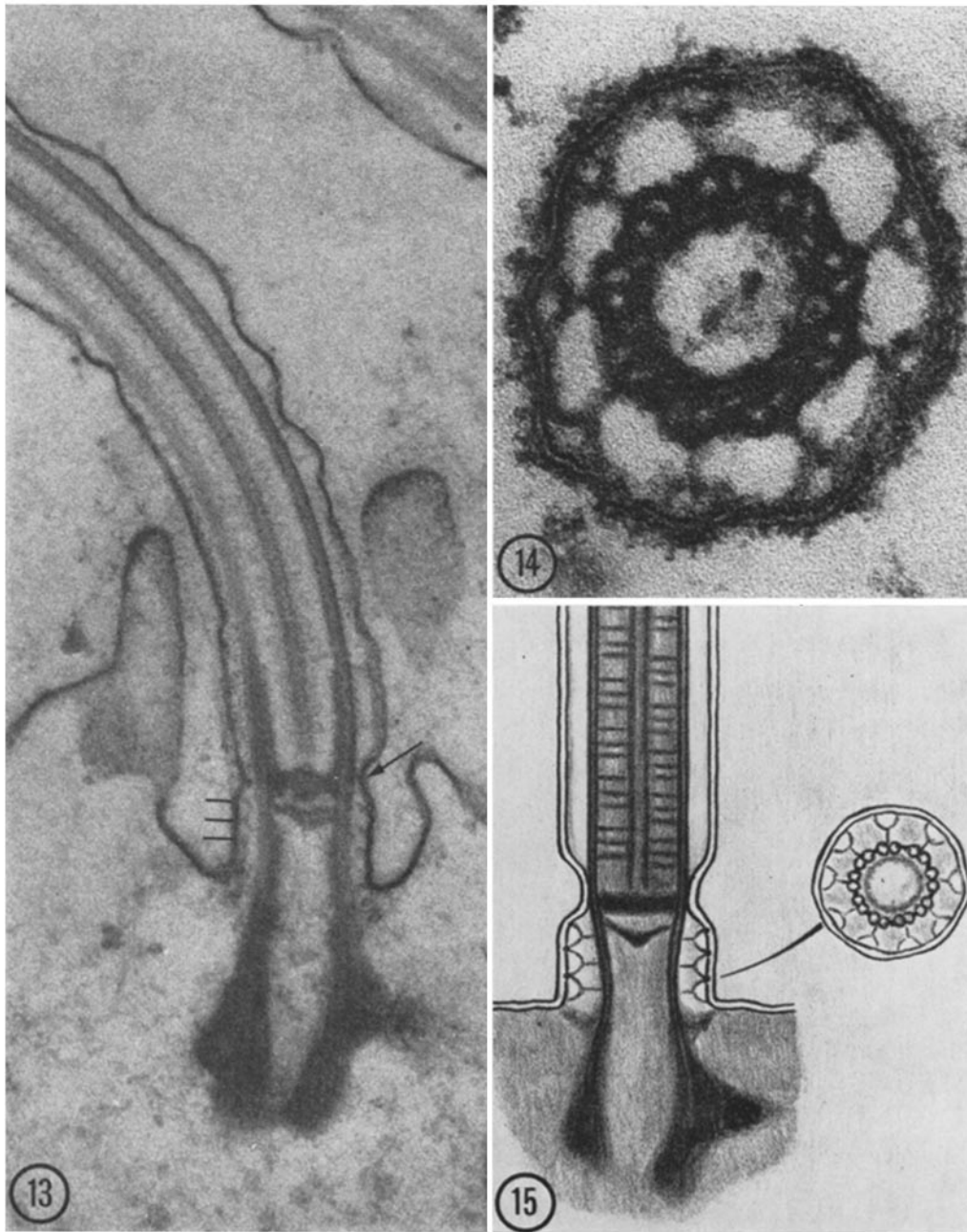
FIGURE 13 Thin section through longitudinal plane of an Elliptio lateral cilium which contains a longitudinal view of the thin-section necklace components. The membrane pinches in at the basal plate (arrow). Below the basal plate, the necklace region contains three bowls or cups (lines) which are apposed against the membrane. \times 80,000 .
