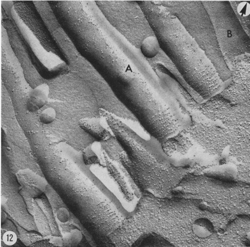
FIGURE 12 Fracture faces ( A and B ) of cilia from rat tracheal epithelium. These cilia contain six particle strands in their necklace region. \times 80,000 .
