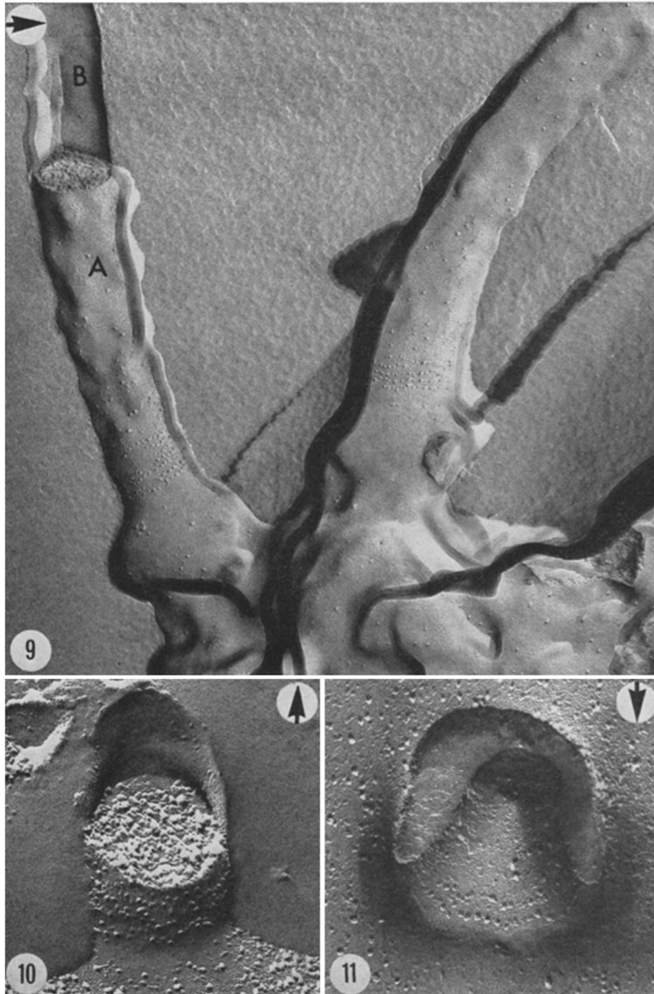
FIGURE 9 Freeze-fracture of two flagella of the ameboflagellate Tetramitus . Few particles are present in the shaft region on either face A (A) or B (B). The necklace region contains a variable number of unscalped particle strands. \times 70,000 .
