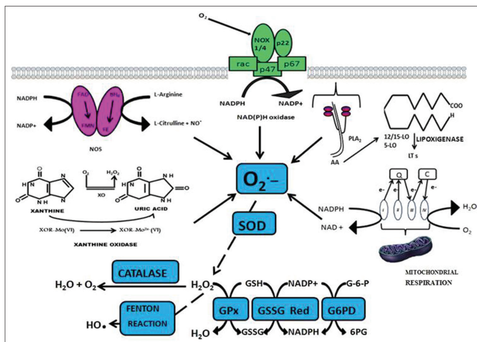
Figure 2: Outline of various sources of reactive oxygen species and action of antioxidant enzymes. Q: Indicates coenzyme Q; C: Cytochrome C; FAD: Flavin adenine dinucleotide; FMN: Flavin mononucleotide; FE: Heme iron; BH4: Tetrahydrobiopterin
