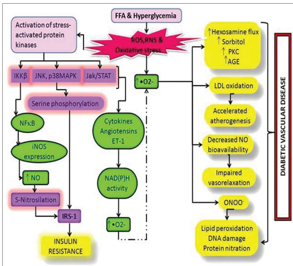
Figure 1: Schematic representation of oxidative stress and the pathways leading to type 2 diabetes mellitus and its complications
