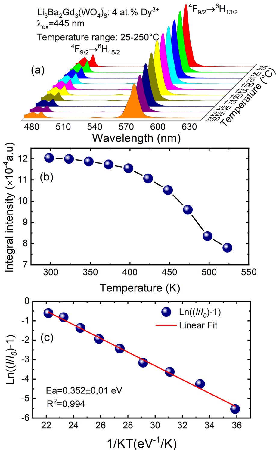
Fig. 10 (a) Emission spectra of samples doped with 4 at% \text{Dy}^{3+} excited at 445 nm under in situ temperature ranging from 25 to 250 °C with a step of 25 °C; (b) integral intensity of the {}^4\text{F}_{9/2} \rightarrow {}^6\text{H}_{13/2} transition as a function of temperature; (c) \ln[(I/I_0)-1] vs. 1/kT activation energy graph for thermal quenching of 4 at% \text{Dy}^{3+} doped quaternary tungstate \text{Li}_3\text{Ba}_2\text{Gd}_3(\text{WO}_4)_8 .
