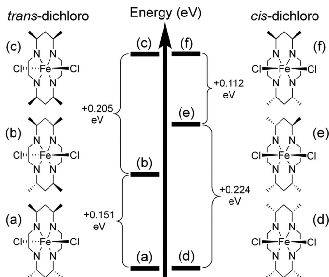
Figure 6 DFT-derived energetic orderings for complexes of various isomers of CTMC in planar (left) or folded (right) conformations.
