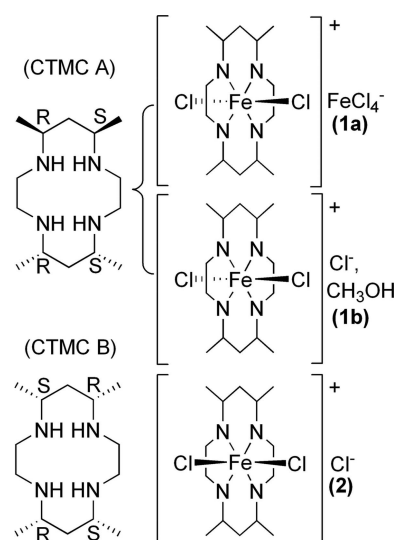
Figure 1 Stereoisomers of CTMC (left) and the resulting iron coordination complexes (right) discussed herein.
