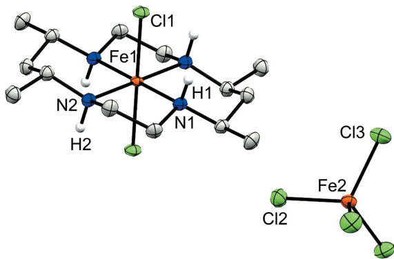
Figure 2 Displacement ellipsoid plot of 1a . H atoms (except for those bound to N atoms) and the minor disordered FeCl 4 − moiety have been omitted for clarity.
