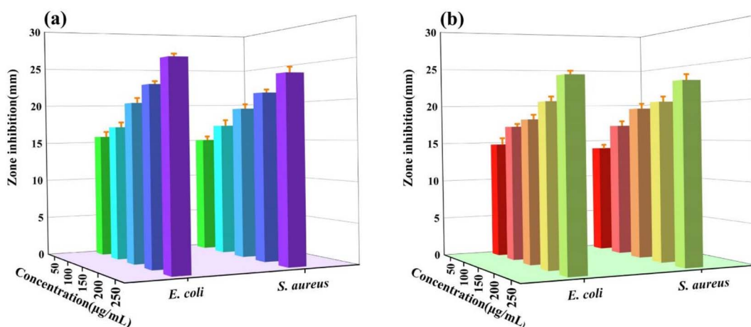
Fig. 4 (a) Complex 1 and (b) complex 2 antibacterial activity against S. aureus ATCC6538 and E. coli ATCC25922.
