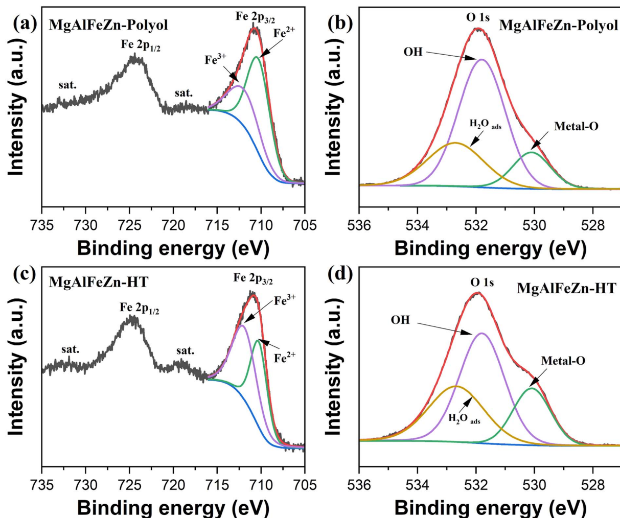
Fig. 7 (a) Fe 2p and (b) O 1s XPS spectra of the MgAlFeZn-polyol. (c) Fe 2p and (d) O 1s XPS spectra of the MgAlFeZn-HT.
