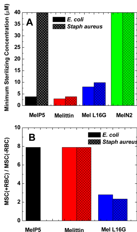
Figure 6. Antibacterial activity. (A) Minimum sterilizing concentrations against E. coli and S. aureus were determined with standard broth dilution assays 40 averaged over at least three independent experiments. Peptide concentrations were serially diluted from 40 μM; thus, any bars at 40 μM indicate a lack of observed activity. (B) MSC measurements were made using broth dilution in which all steps were done in the presence of 1 \times 10^9 erythrocytes (RBCs) per mL. The Y-axis is the ratio of the MSC in the presence of erythrocytes to the MSC in their absence.
