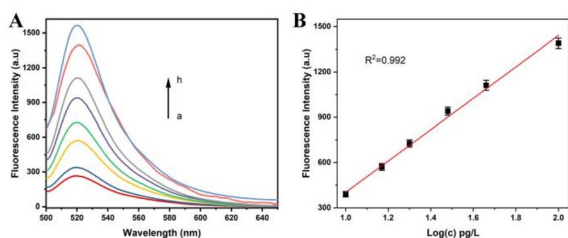
Fig. 3 (A) Fluorescence intensity of the solutions at different genome concentrations of A. alternata . Arrow from a to h represents the genome concentrations of 0 pg L^{-1} , 10 pg L^{-1} , 15 pg L^{-1} , 20 pg L^{-1} , 30 pg L^{-1} , 50 pg L^{-1} , 0.1 ng L^{-1} , and 0.2 ng L^{-1} . (B) Linear correlation between fluorescence intensity and logarithm of A. alternata genome concentration from 10 pg L^{-1} to 0.1 ng L^{-1} . Pg means picogram, and ng means nanogram.
