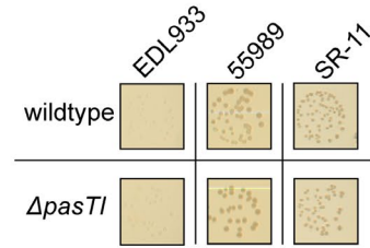
(b) colony size of different E. coli / Salmonella strains under anaerobic conditions
