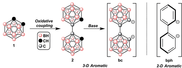
Fig. 1 Oxidative coupling of o -carborane ( 1 ) yields 1,1'-bis( o -carborane) ( 2 ), 10a effectively a 3D analogue of biphenyl (Fig. 1), and in 1973, Zakharkin showed that the oxidative coupling of two o -carboranes ( 1 ) through carbon vertices yields 2 . 10d Later, Hawthorne demonstrated that the deprotonation of 2 results in a dianionic species bc , which was shown to bind several transition metals in bidentate or monodentate fashions. 10b-f Ligand bc possesses similar electronic and physical properties as the parent o -carborane (see ESI†), and behaves as a robust transition metal ligand. More recently, several groups have improved the synthesis of 2 (ref. 10j) and further expanded the series of heteroleptic late-transition metal complexes containing bc . 11 However, fundamental electronic characterization and potential applications for these compounds as electronic materials have yet to be disclosed.
