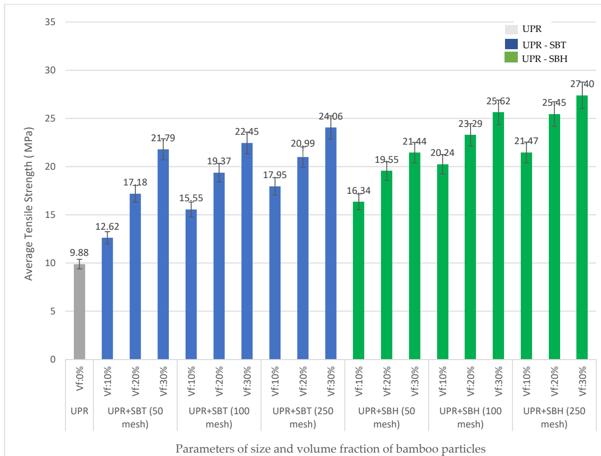
Figure 9. Relationship between volume fraction on the particle size of SBT and SBH polyester (UPR) matrix on tensile strength.
